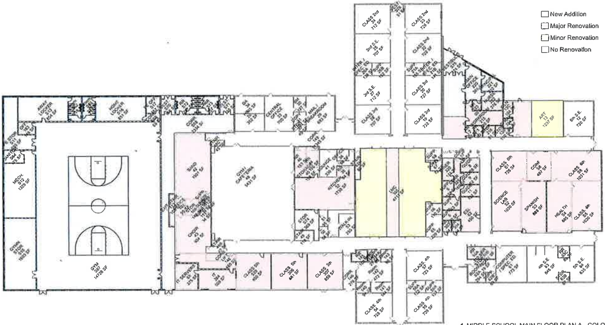
1 MIDDLE SCHOOL MAIN FLOOR PLAN A - COLOR CODED SCALE 1" = 30'
